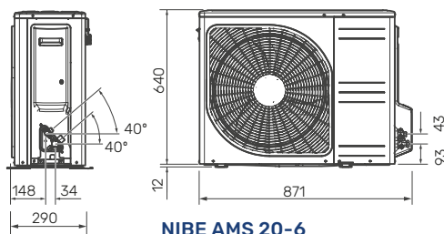
NIBE AMS 20-6
