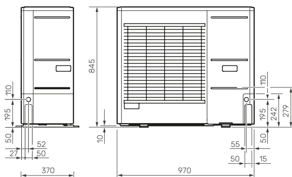
NIBE AMS 10-12
