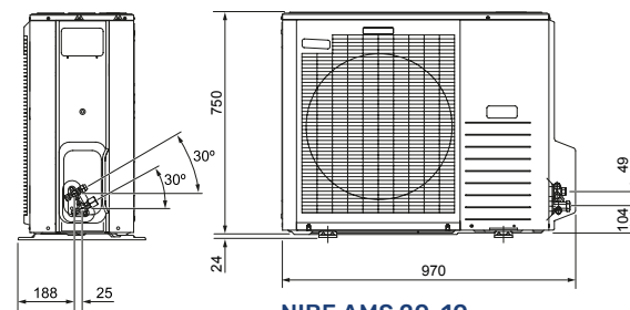
NIBE AMS 20-10
