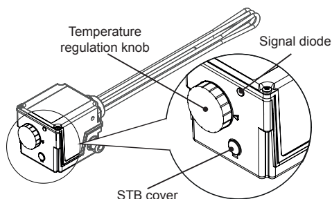
Fig. 8 Front of the ME 0040 / ME 1045 / ME 1060 / ME 1090 / ME 2090 / ME 2120 / ME 2180 module housing.
