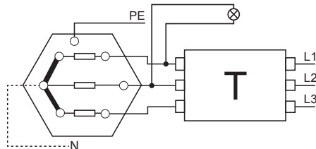
Fig. 5 Electrical diagram ME 0040 - ME 2090.
