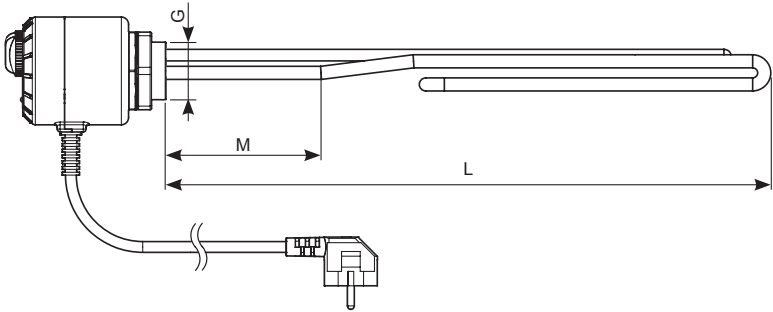
Fig. 9. ME 1030 heating module.
