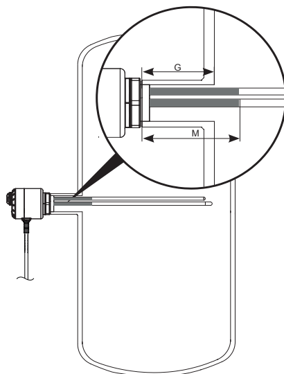
Fig. 3 The correct depth of the connection pipe.
