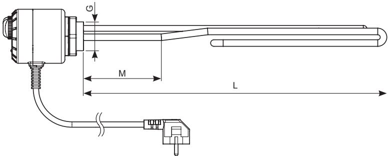
Ritning. 9. Elpatron ME 1030.
