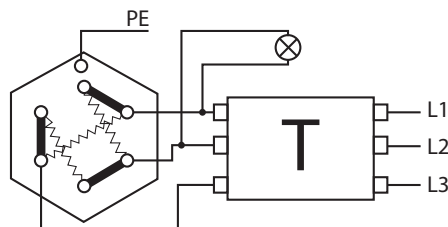
Fig. 6 Electrical diagram ME 2120 - ME 2180.
