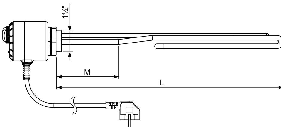
Fig. 8. ME 0020 and ME 0030 Geometrical data.
