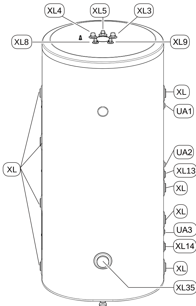
Rys. 3 BUZ - 400/150.92N
